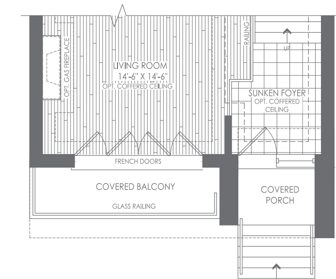
PARTIAL SECOND FLOOR ELEV. B
