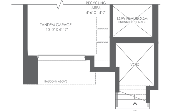
PARTIAL GROUND & OPT. GROUND FLOOR ELEV. B
