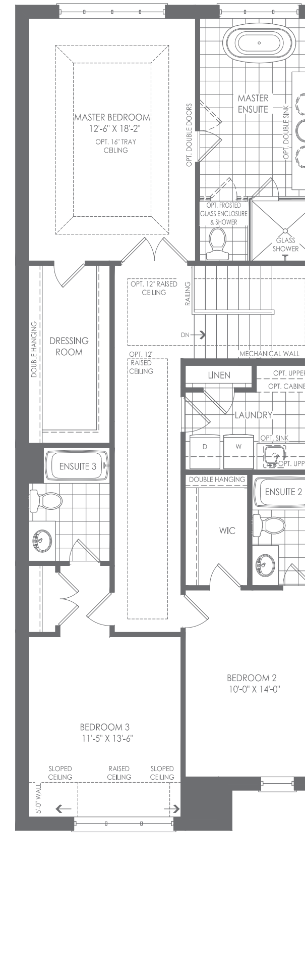
THIRD FLOOR ELEV. A
