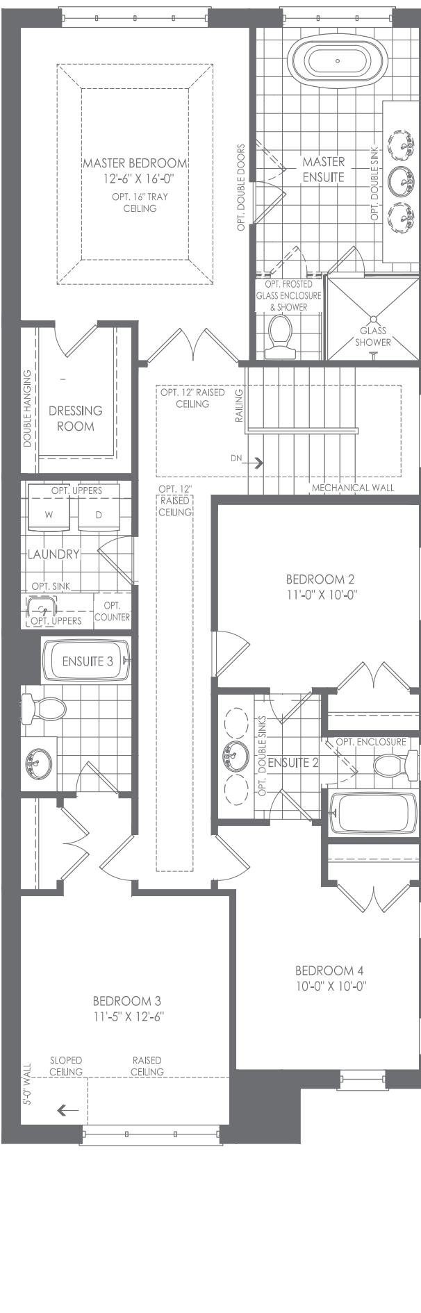
OPTIONAL THIRD FLOOR ELEV. A 4 BEDROOM PLAN
